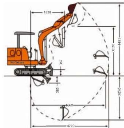
Dimensions with optional attachment
