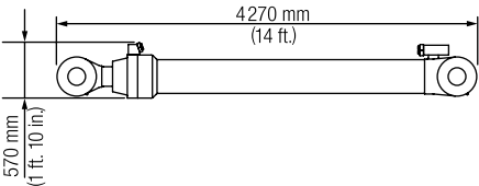
BOOM CYLINDER Weight: 2270 kg (5,004 lb.)
