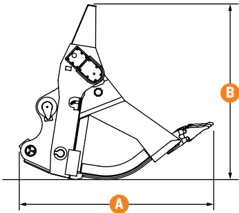
BUCKET ASSEMBLY
