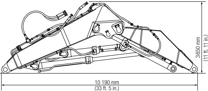
BOOM AND ARM ASSEMBLY Weight: 25 260 kg (55,689 lb.) Width: 2160 mm (7 ft. 1 in.)
