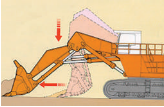
Auto-Leveling Crowd Mechanism
