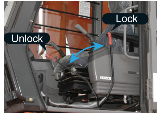
Pilot-Control Shut-off Lever
